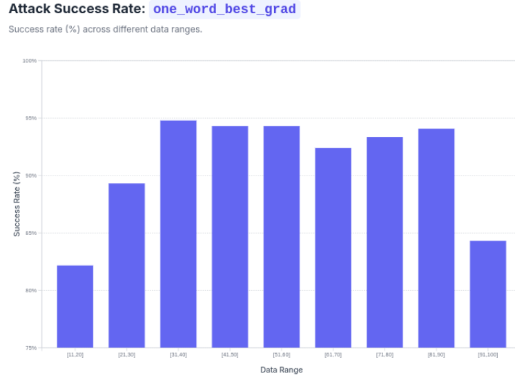
FIGURE 4.1: Interval success rate of one_word_best_grad method on BERT-base-mdoc-BM25, trec-dl-2019 queries, data from Table 4.3.
