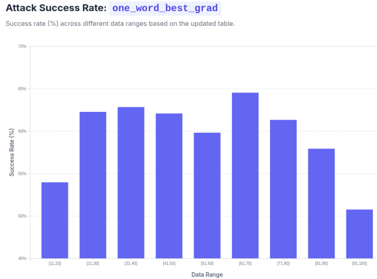
FIGURE 4.2: Interval success rate of one_word_best_grad method on monoT5-base-MSMARCO, trec-dl-2020 queries, data from Table 4.11.
