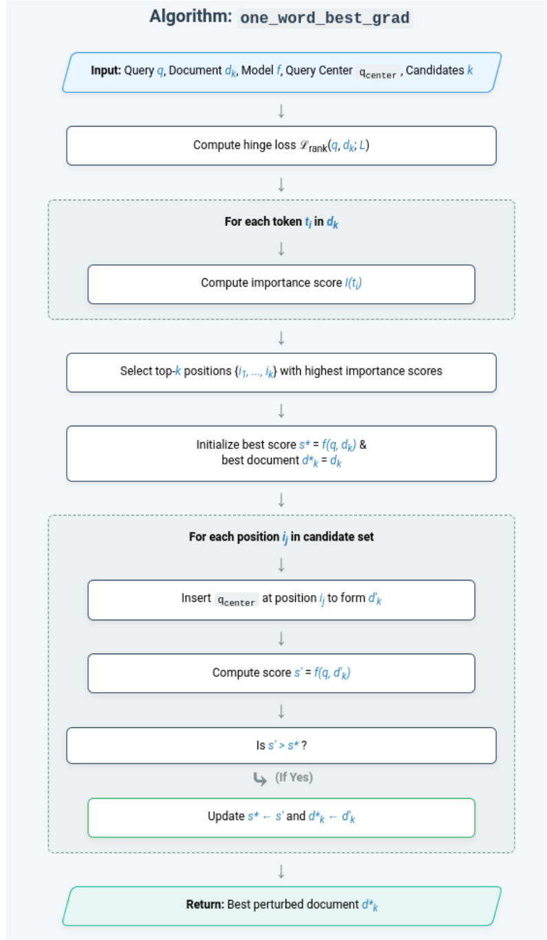
FIGURE 3.1: one_word_best_grad framework
